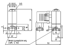
Electro-valve 2/2
