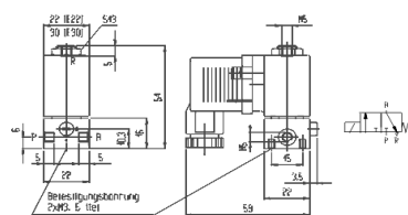
Electro-valve 3/2
